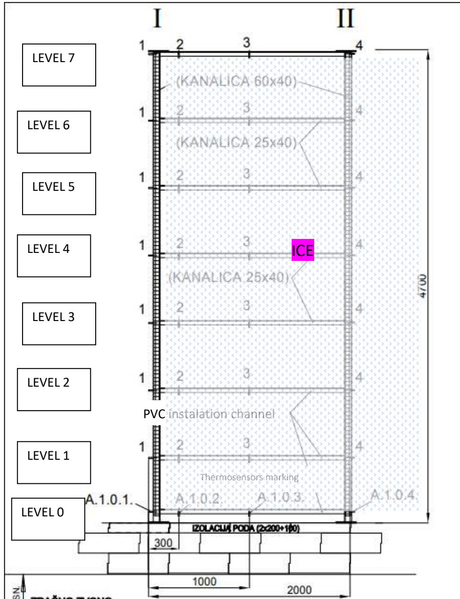
A 1 measuring point ( 32 sensors)
